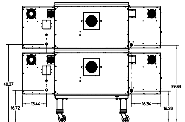
PS640 Back View – Gas Double Stacked w/Legs
